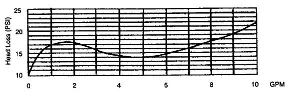
Model 820 (1/4", 3/8", 1/2") Flow Curve
