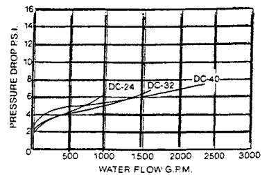
Lawler Double Check Backflow Preventer
