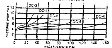
Lawler Double Check Backflow Preventer
