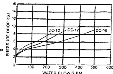
Double Check (DC)
