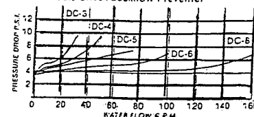
Lawler Double Check Backflow Preventer
