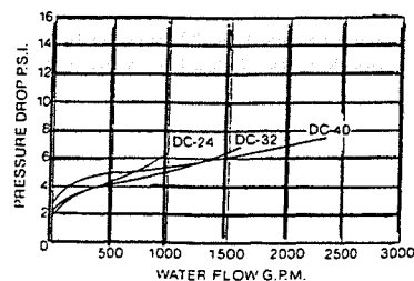
Lawler Double Check Backflow Preventer
